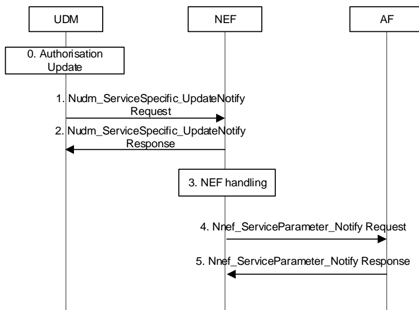
Figure 4.15.6.10-2: Service Specific Authorization Update procedure
