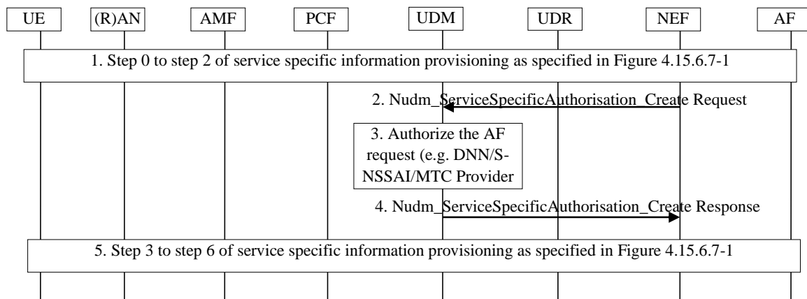
Figure 4.15.6.10-1: Service Specific Authorization for an individual UE or group of UEs
