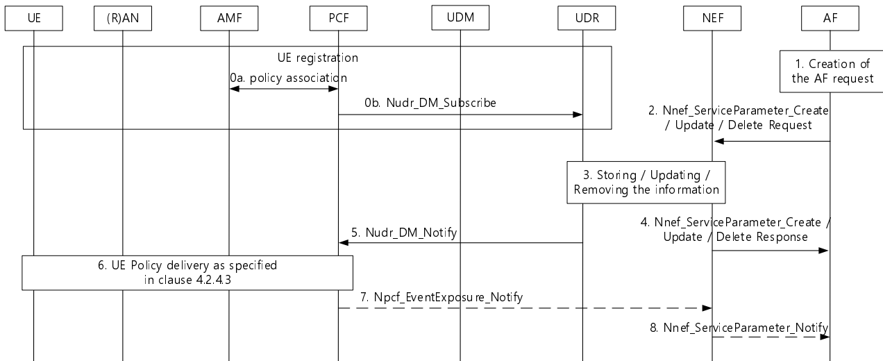
Figure 4.15.6.7-1: Service specific information provisioning
