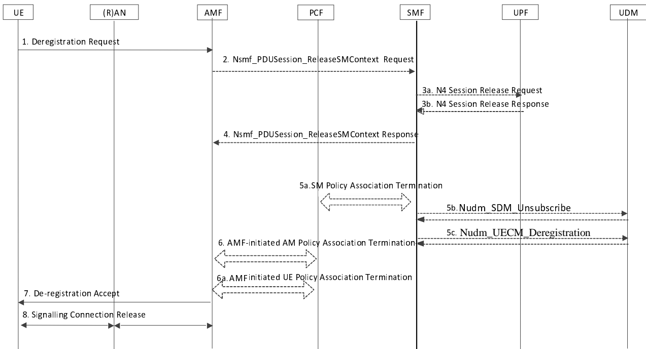
Figure 4.2.2.3.2-1: UE-initiated Deregistration
