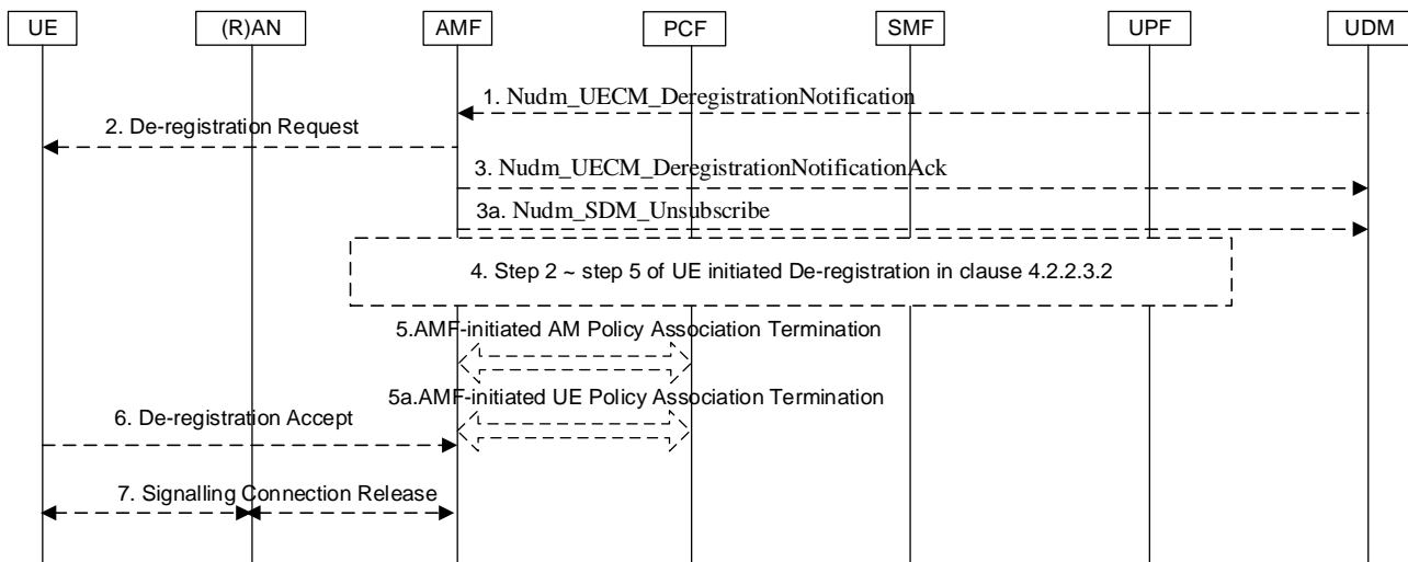
Figure 4.2.2.3.3-1: Network-initiated Deregistration
