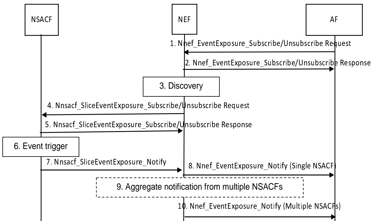
Figure 4.15.3.2.10-1: Number of UEs and PDU Sessions per network slice notification procedure
