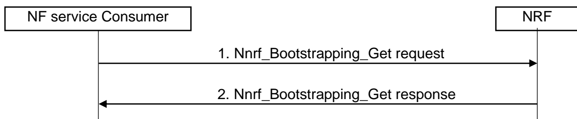
Figure 4.17.13-1: Bootstrapping procedure
