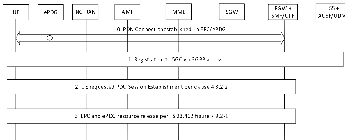
Figure 4.11.4.1-1: Handover from EPC/ePDG to 5GS
