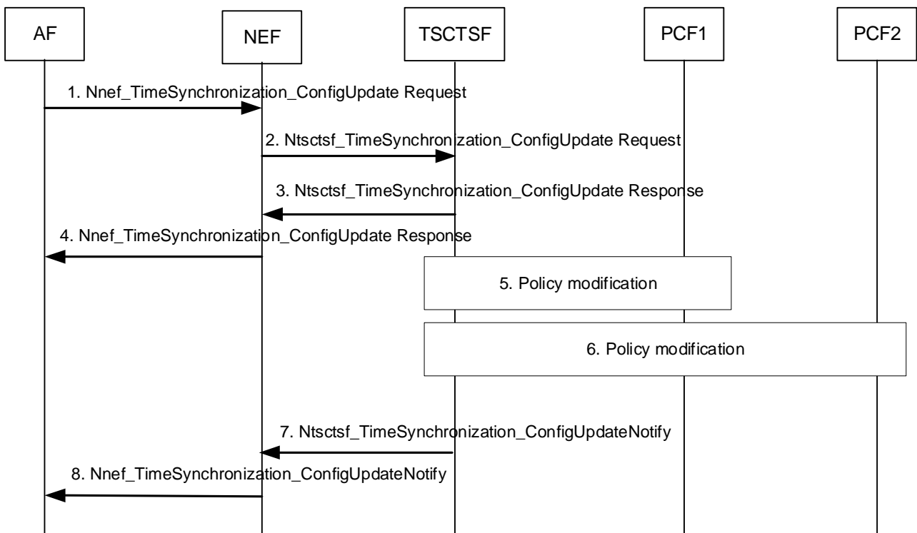
Figure 4.15.9.3.3-1: Time synchronization service modification
