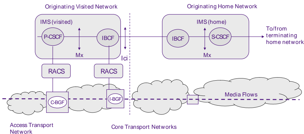
Figure 6: IMS interconnect scenario with I-BGF
