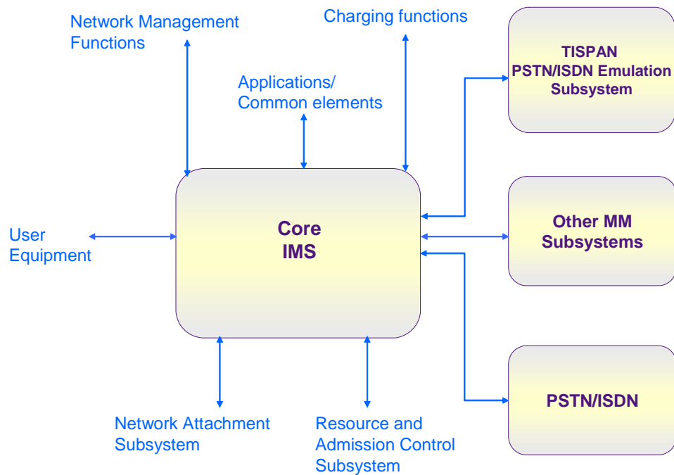
Figure 2: TISPAN IMS and its environment
