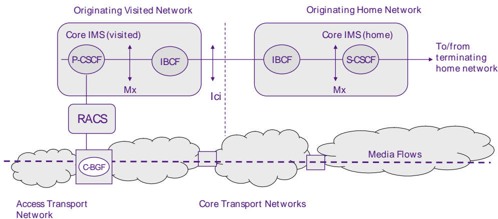
Figure 5: IMS interconnect scenario without I-BGF
