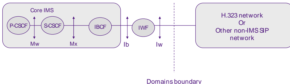
Figure B.5: Interworking with non-IMS multimedia networks
