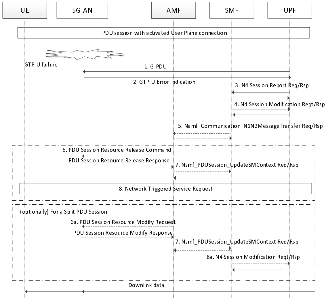
Figure 5.3.2.1-1: GTP-U Error Indication from 5G-AN
