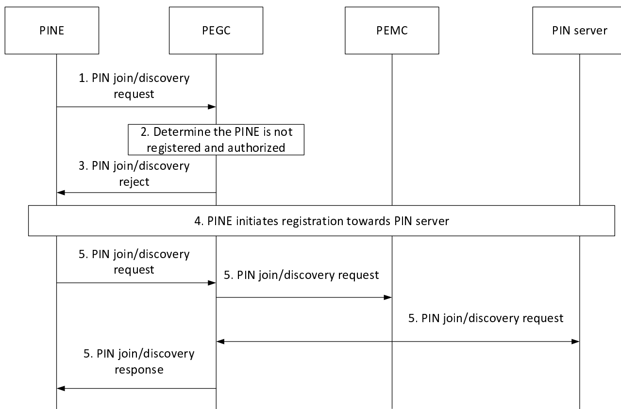
Figure 8.4.2.2.4-1: PINE registration to PIN server during PIN join via PEGC
