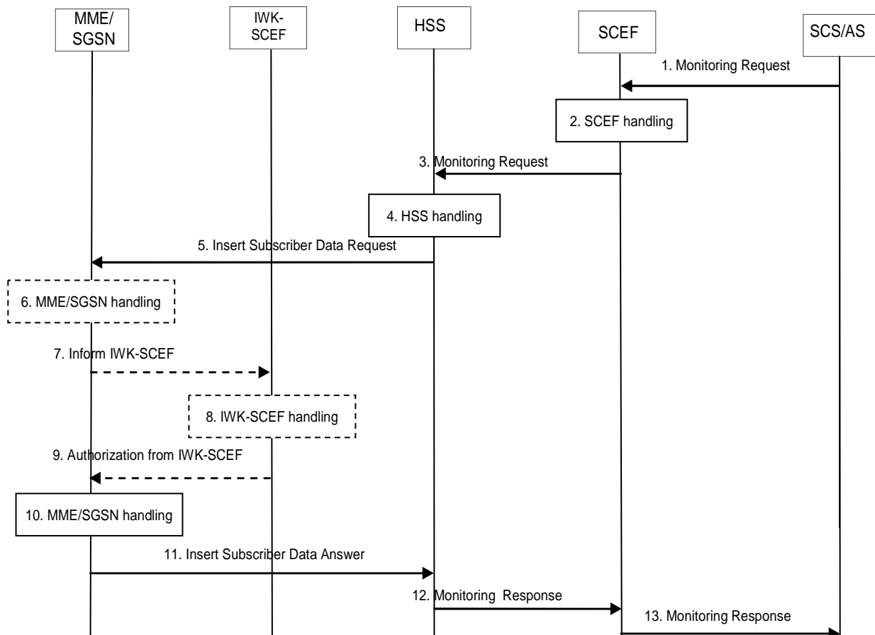
Figure 5.6.6.1-1: Monitoring event configuration and deletion via HSS procedure
