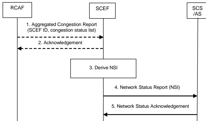
Figure 5.8.3-1: Report procedure for continuous reporting of network status
