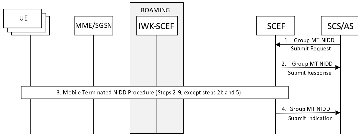
Figure 5.5.3-1: Group Message Delivery via unicast MT NIDD
