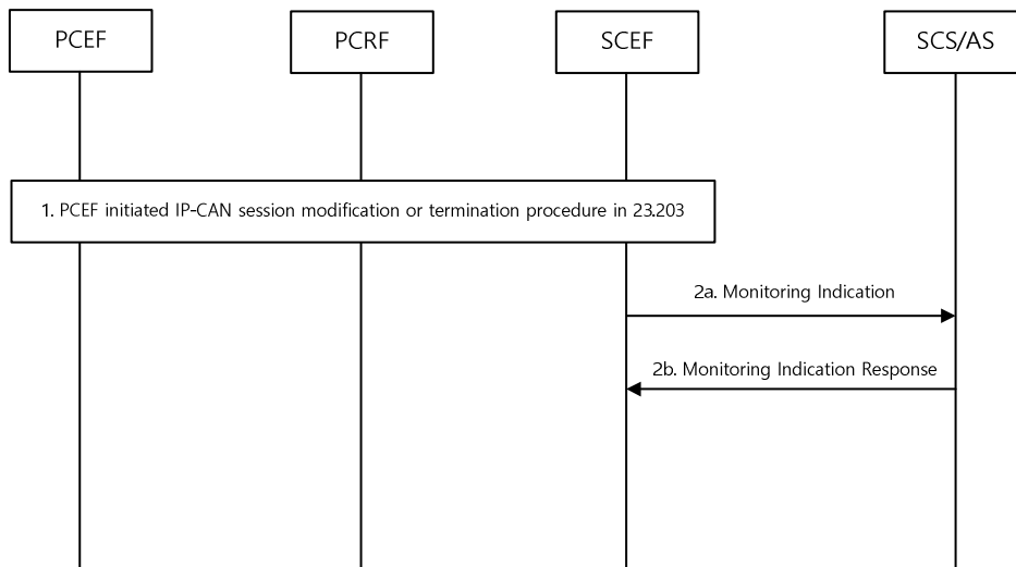
Figure 5.6.5-1: Reporting event procedure
