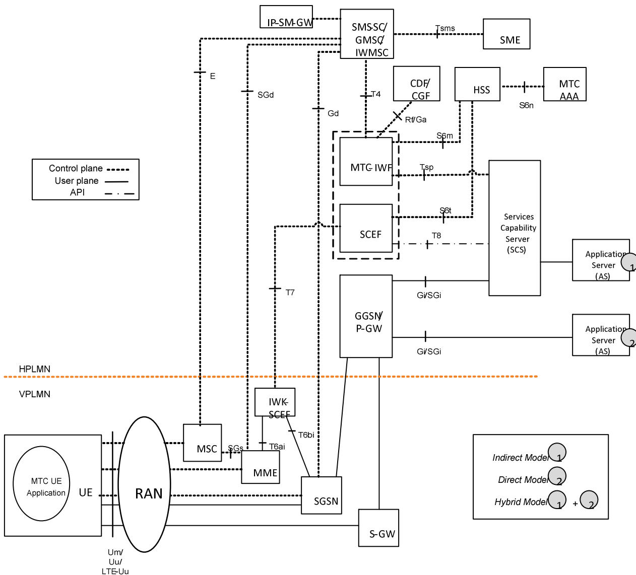
Figure 4.2-1b: 3GPP Architecture for Machine-Type Communication (Roaming)
