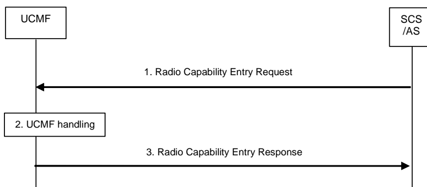
Figure 5.19.3-1: RACS information provisioning procedure via T9a
