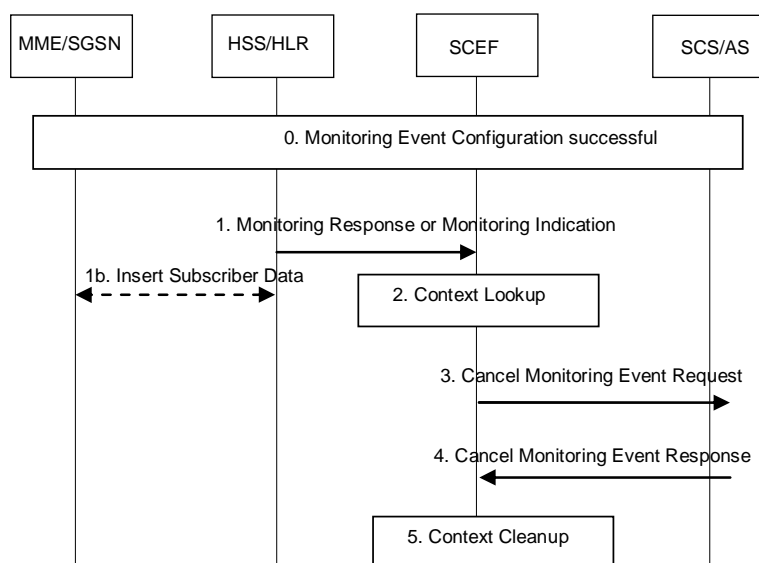
Figure 6.5.9-1: Network-initiated Explicit Monitoring Event Deletion Procedure
