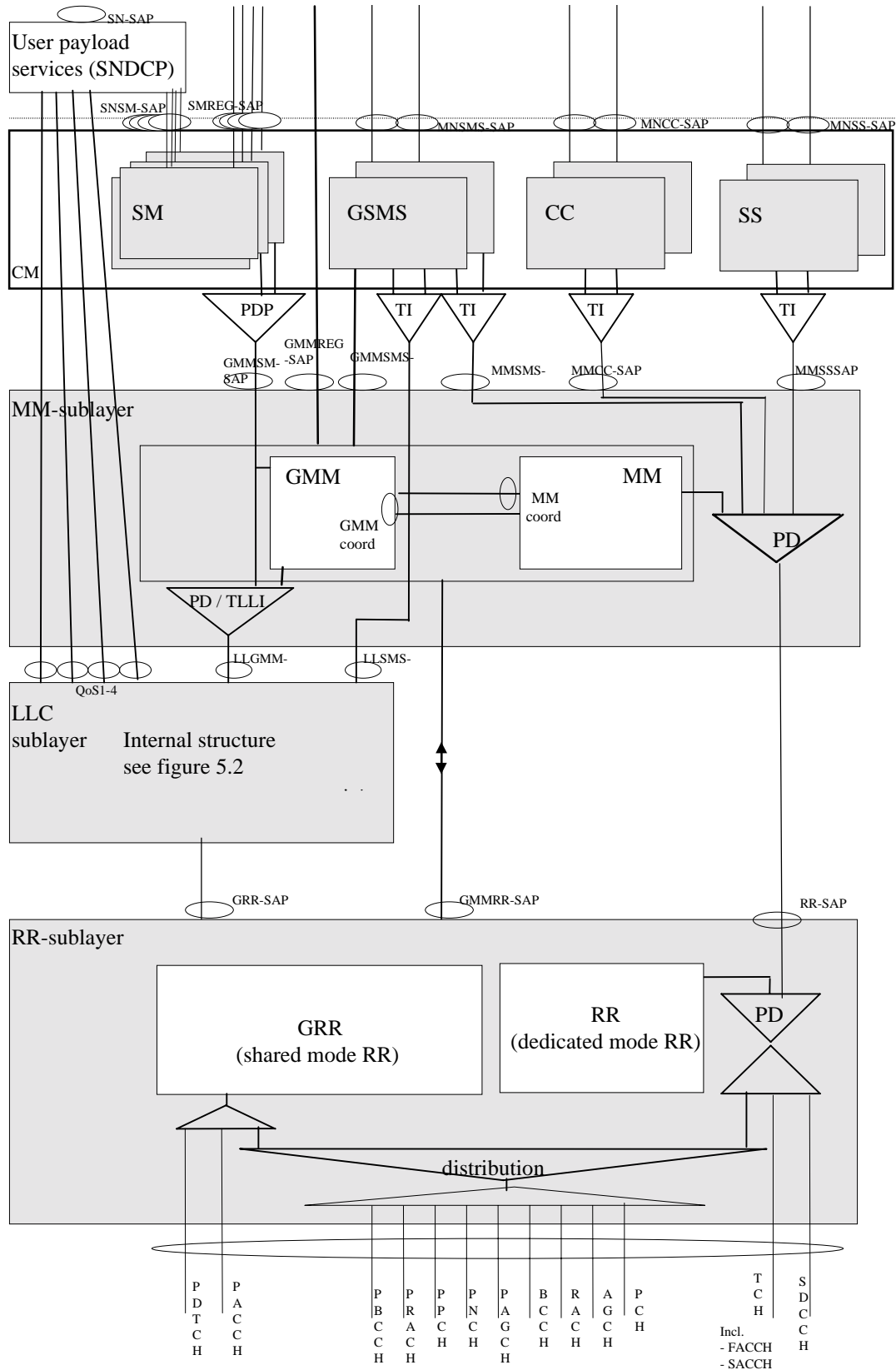
Figure 5.3/TS 24.007: Protocol architecture supporting GPRS class A and B MSs, MS - side
