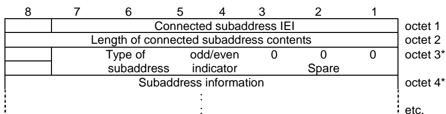
Figure 10.5.100/3GPP TS 24.008
