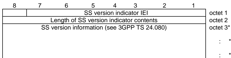
Figure 10.5.113/3GPP TS 24.008
