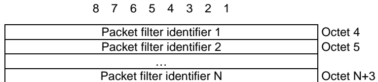
Figure 10.5.144a/3GPP TS 24.008: Packet filter list when the TFT operation is "delete packet filters from existing TFT" (z=N+3)
