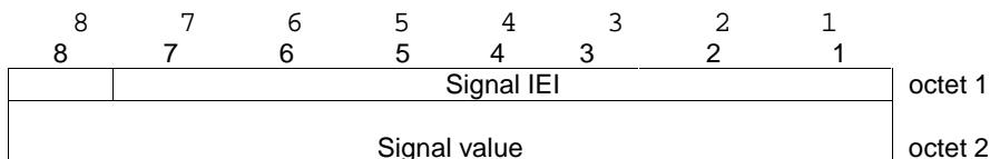
Figure 10.5.112/3GPP TS 24.008 Signal information element
