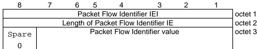
Figure 10.5.143/3GPP TS 24.008: Packet Flow Identifier information element
