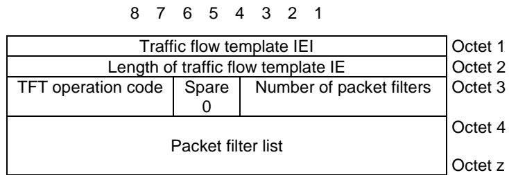
Figure 10.5.144/3GPP TS 24.008: Traffic flow template information element
