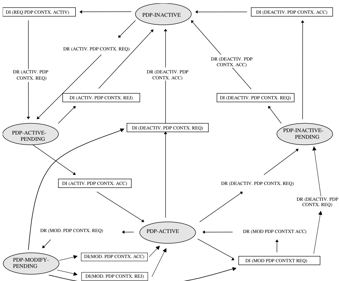
Figure 6.1/3GPP TS 24.008: Session management states in the MS (overview)
