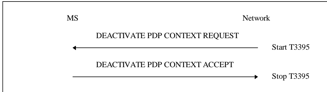
Figure 6.11/3GPP TS 24.008: MBMS context deactivation procedure
