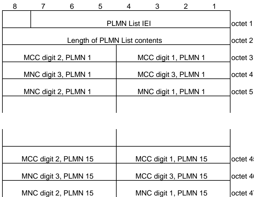
Figure 10.5.13/3GPP TS 24.008 PLMN List information element
