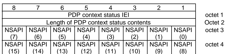
Figure 10.5.148/3GPP TS 24.008 PDP context status information element
