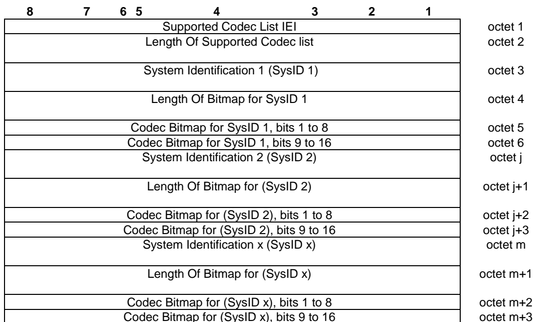
Figure 10.5.118c/3GPP TS 24.008 Supported codec list information element
