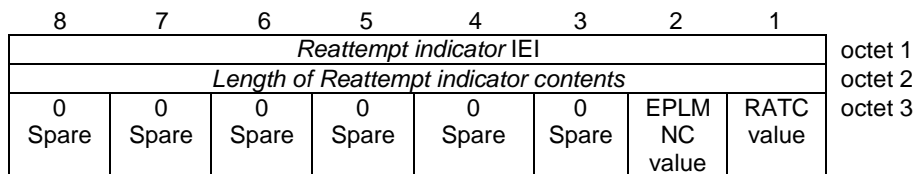
Figure 10.5.6.5A: Re-attempt indicator information element
