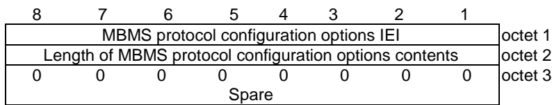
Figure 10.5.156/3GPP TS 24.008: MBMS protocol configuration options information element
