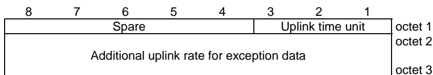
Figure 10.5.6.3.3-1B/3GPP TS 24.008: Additional APN rate control parameters for exception data
