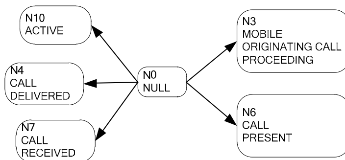
Figure 5.1b.2/3GPP TS 24.008: Overview call control protocol/Network side, extension for SRVCC from PS to CS
