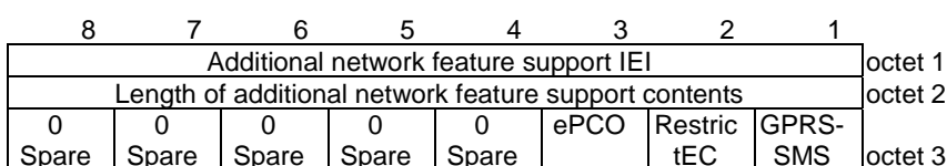
Figure 10.5.5.23A: Additional network feature support information element
