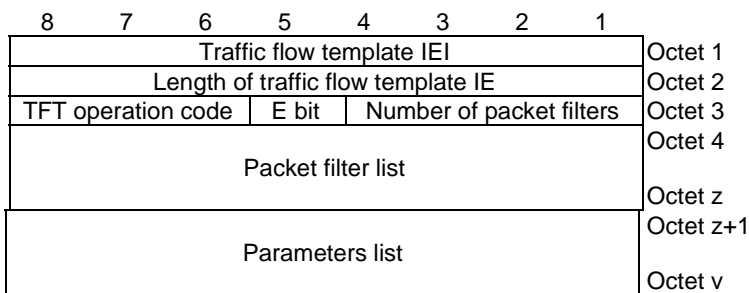
Figure 10.5.144/3GPP TS 24.008: Traffic flow template information element
