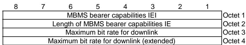
Figure 10.5.155/3GPP TS 24.008: MBMS bearer capabilities information element
