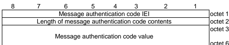
Figure 10.5.5.33-1/3GPP TS 24.008: Message authentication code information element
