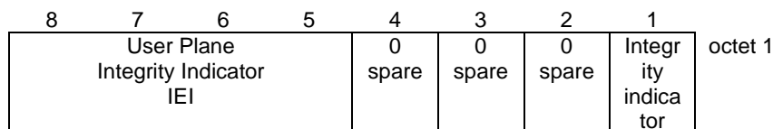
Figure 10.5.5.34-1/3GPP TS 24.008 User Plane integrity indicator information element
