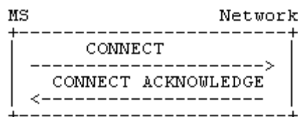
Figure 5.7/3GPP TS 24.008 Call acceptance and active indication at mobile terminating call establishment
