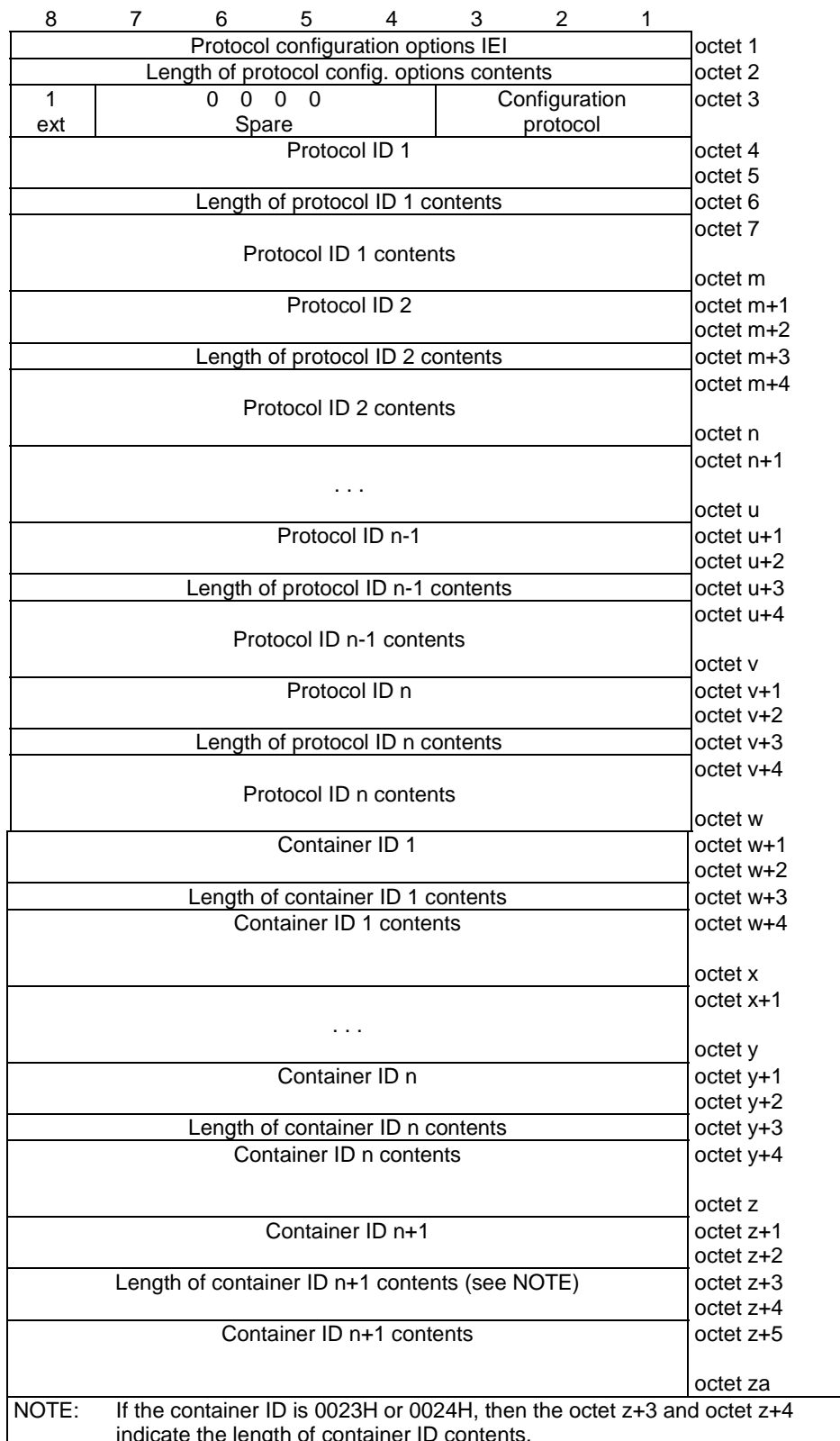
Figure 10.5.136/3GPP TS 24.008: Protocol configuration options information element
