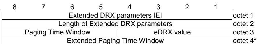
Figure 10.5.5.32/3GPP TS 24.008: Extended DRX parameters information element
