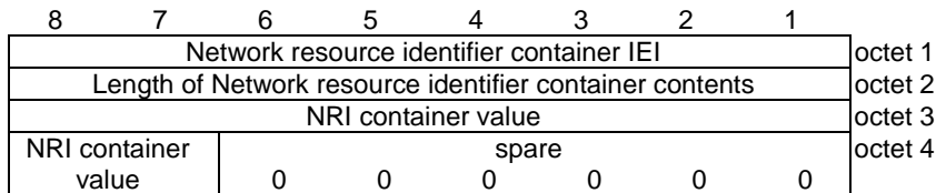
Figure 10.5.5.31/3GPP TS 24.008 Network resource identifier container information element
