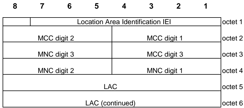
Figure 10.5.3/3GPP TS 24.008 Location Area Identification information element
