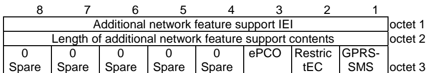
Figure 10.5.5.23A: Additional network feature support information element
