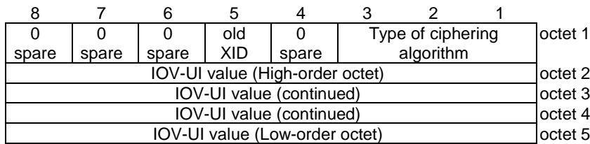
Figure 10.5.1.14/3GPP TS 24.008 NAS container for PS HO information element
