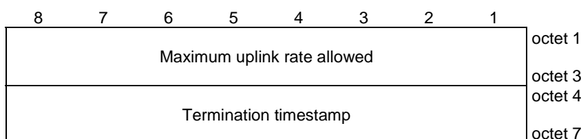
Figure 10.5.6.3.6-1/3GPP TS 24.008: Initial small data rate control parameters
