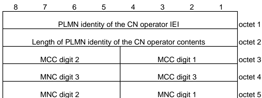
Figure 10.5.5.36-1/3GPP TS 24.008 PLMN identity of the CN operator information element
