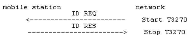
Figure 4.3/3GPP TS 24.008: Identification sequence
