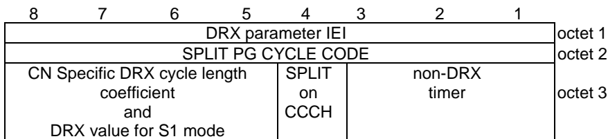
Figure 10.5.122/3GPP TS 24.008: DRX parameter information element
