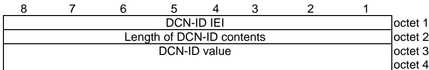
Figure 10.5.5.35-1/3GPP TS 24.008: DCN-ID information element
