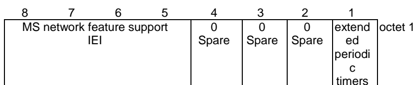
Figure 10.5.1.15/3GPP TS 24.008: MS network feature support information element
