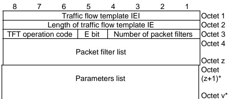
Figure 10.5.144/3GPP TS 24.008: Traffic flow template information element
