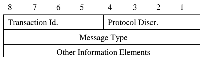
Figure 8.1/TS 24.011
