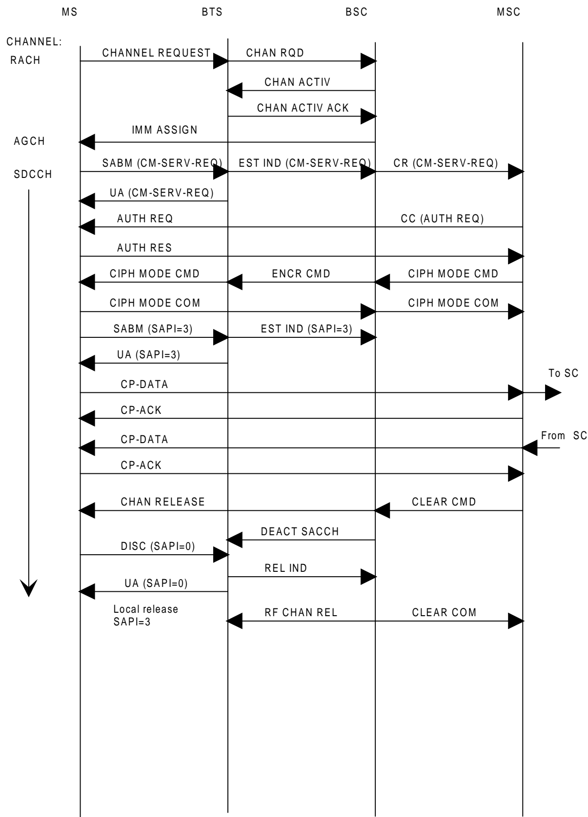
Figure F1/TS 24.011: Mobile originated Short Message on SDCCH
