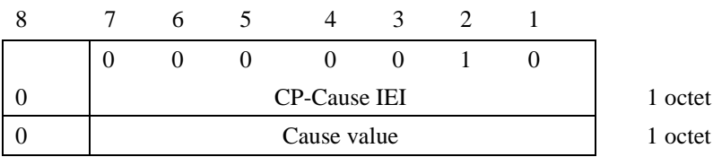
Figure 8.3/TS 24.011: CP-Cause element layout
