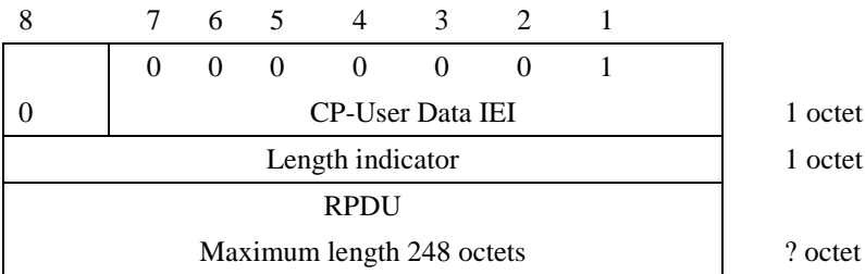
Figure 8.2/TS 24.011: CP-User data element layout
