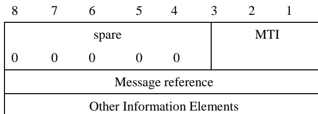
Figure 8.4/TS 24.011
