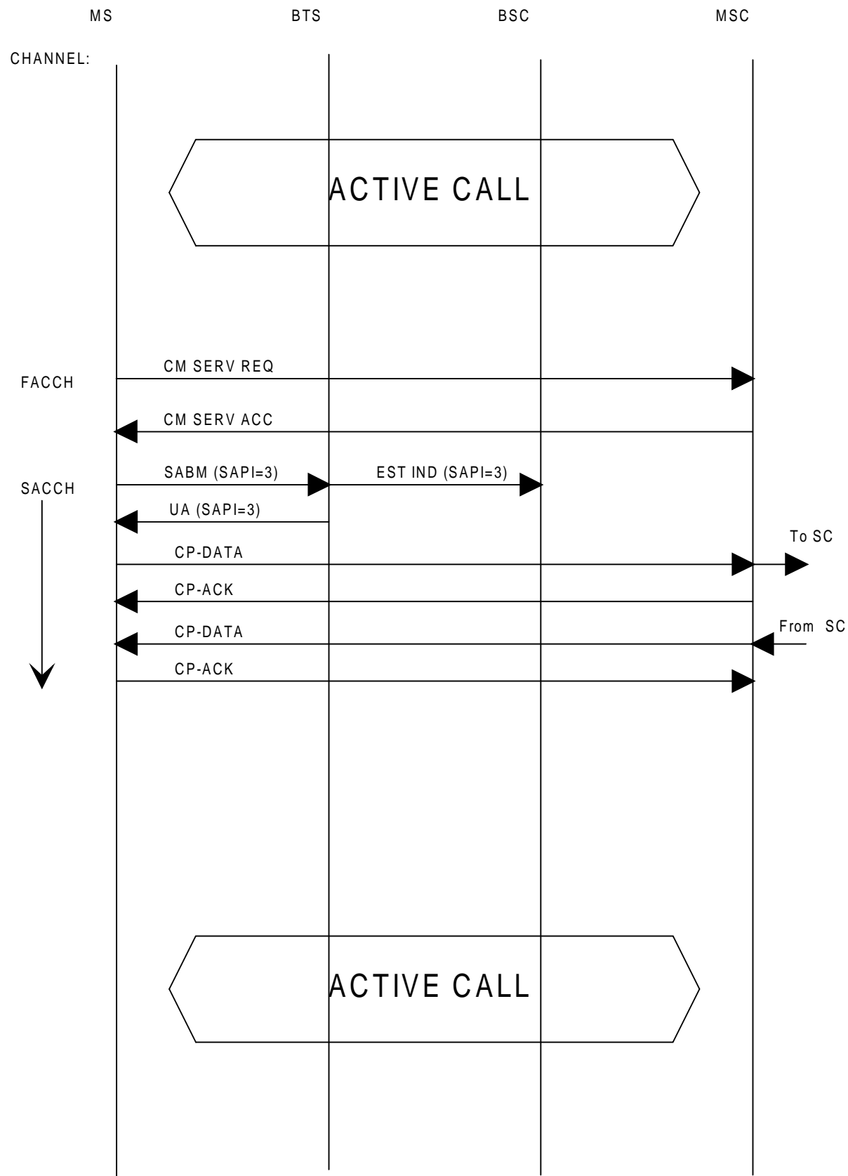
Figure F3/TS 24.011: Mobile originated Short Message on SACCH
