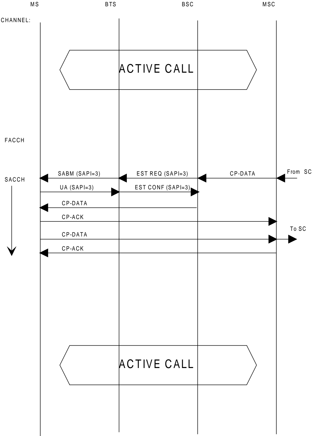
Figure F4/TS 24.011: Mobile terminated Short Message on SACCH
