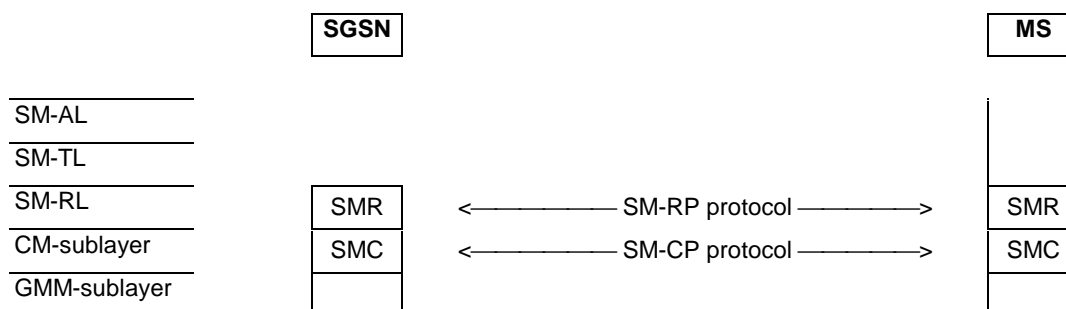
Figure 2.1b/3GPP TS 24.011: Protocol hierarchy for GPRS in A/Gb mode
