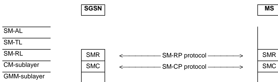
Figure 2.1c/24.011: Protocol hierarchy for packet switched service in lu mode
