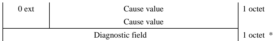
Figure 8.8/3GPP TS 24.011: RP-Cause element layout
