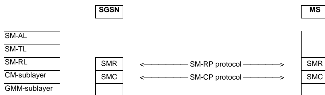
Figure 2.1c/3GPP TS 24.011: Protocol hierarchy for packet switched service in lu mode
