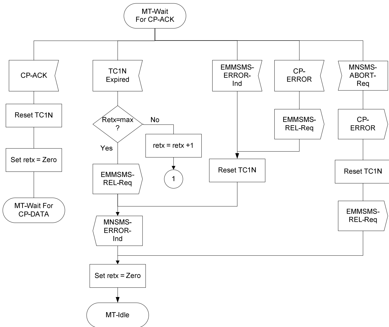
MT-SMC-EP entity on Network-side for EPS when packet-switched service is used SDL-29
