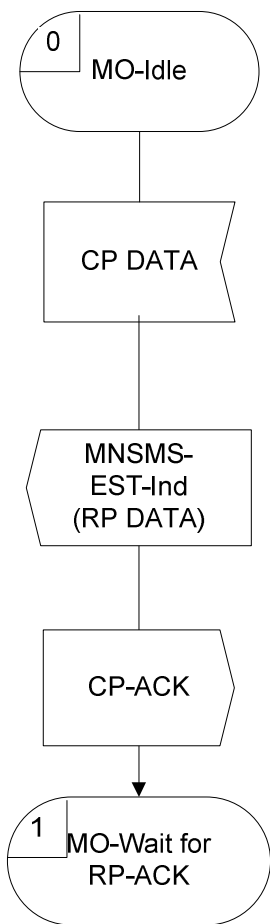
MO-SMC-5G entity on Network side for 5GS when packet-switched service is used SDL-37
