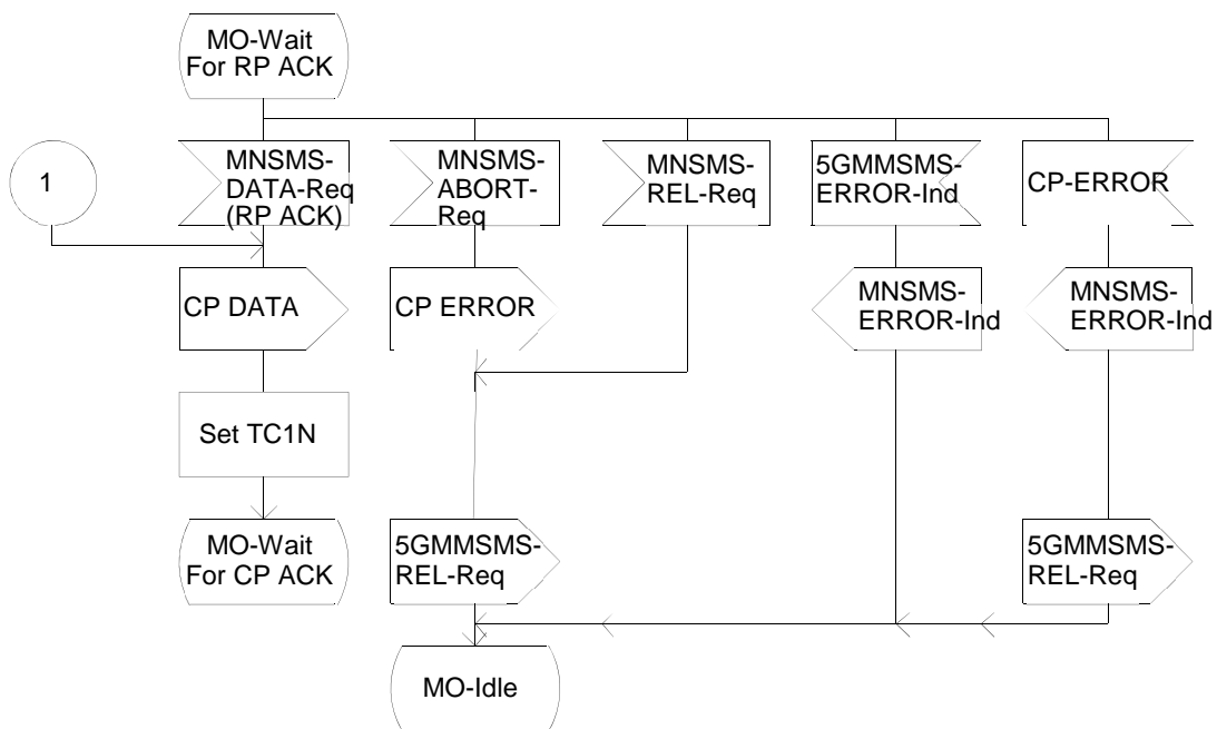
MO-SMC-5G entity on Network side for 5GS when packet-switched service is used SDL-37
