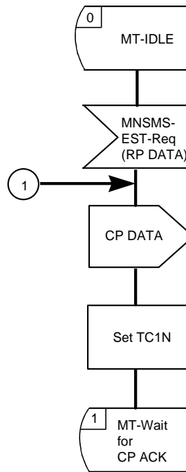
MT-SMC-GP entity on Network-side for GPRS SDL-22
