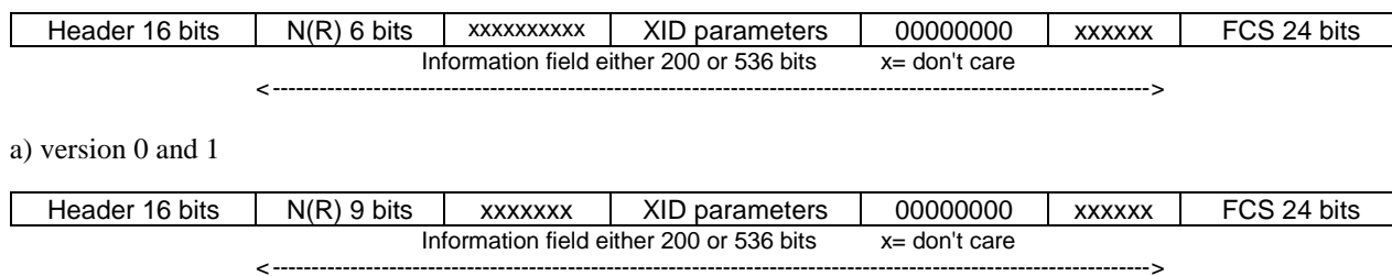
Figure 3: REMAP U-frame format
