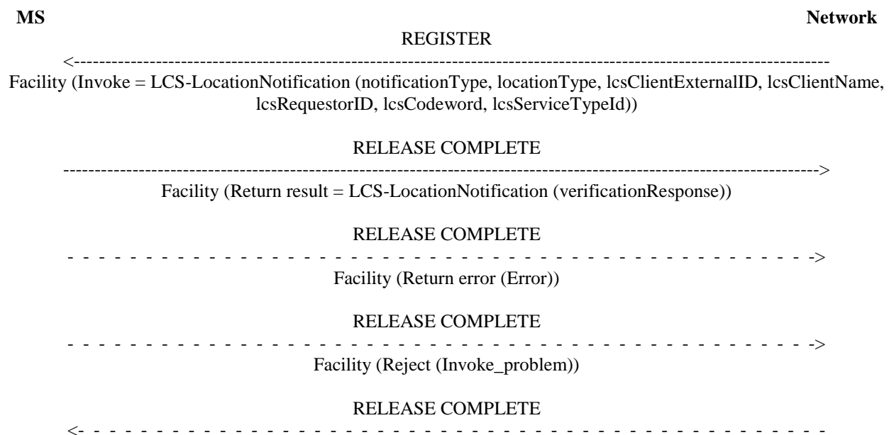
Figure 4.1: Location Notification
