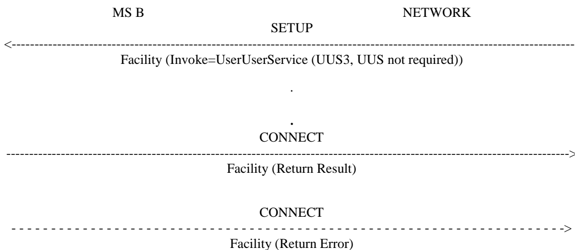
Figure 17: Request for explicit activation of UUS3 when originating a call, UUS not required
