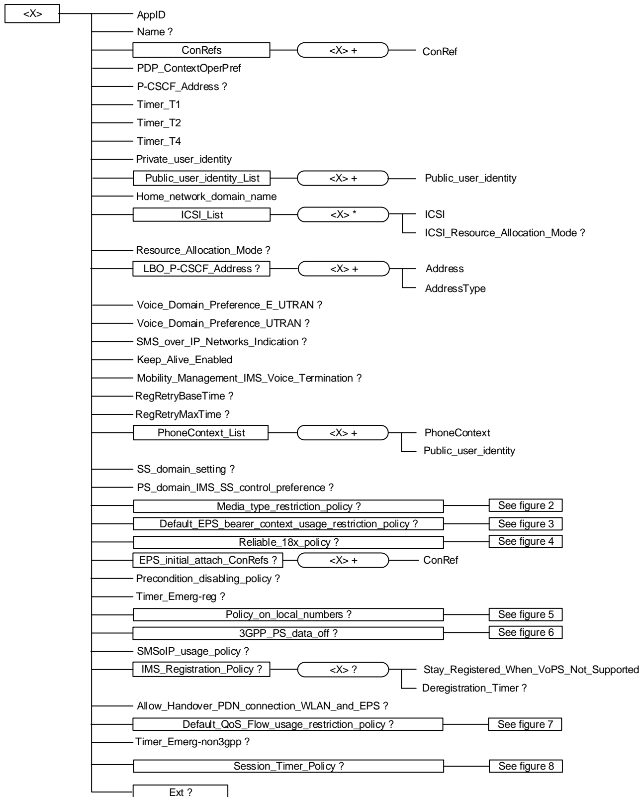
Figure 1: The 3GPP IMS Management Object
