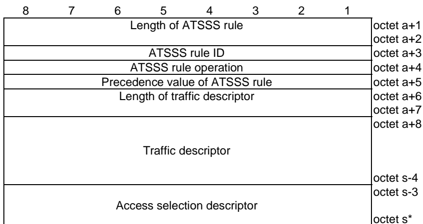
Figure 6.1.3.2-2: ATSSS rule
