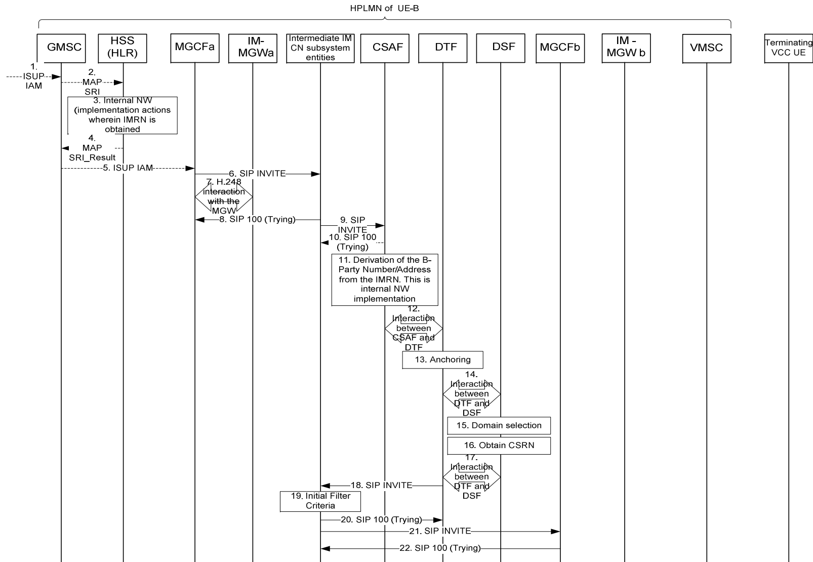
Figure A.5.7-1: Terminating call coming in through CS domain, CS domain selected for call delivery, call delivery unsuccessful, domain for call delivery reselected
