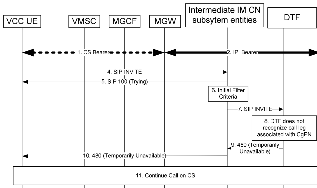
Figure A.6.3-1: Unsuccessful scenario when transferring call from CS to IM CN subsystem
