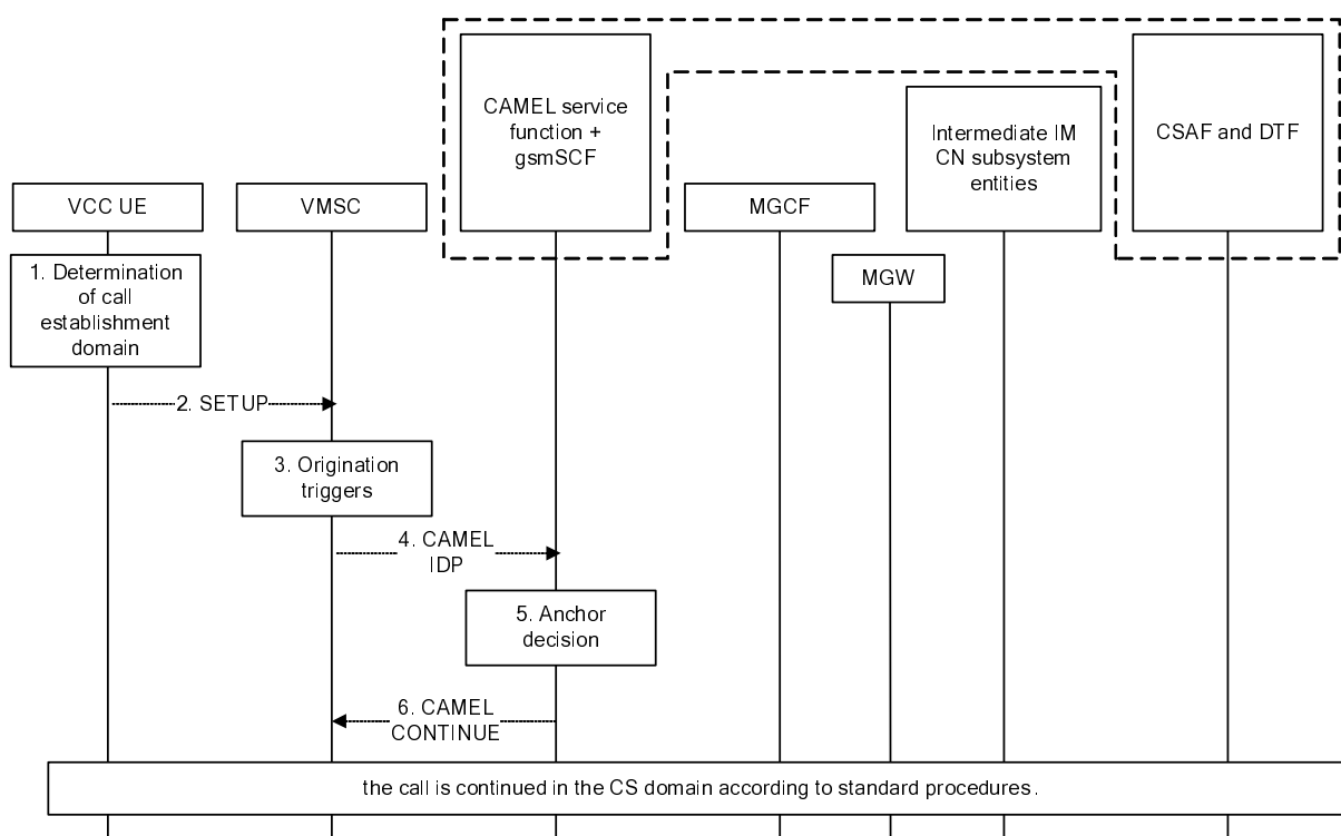
Figure A.4.5-1: call origination from CS with no anchoring
