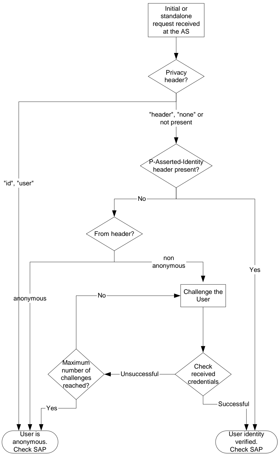
Figure 5-1: User identity verification flow at the AS
