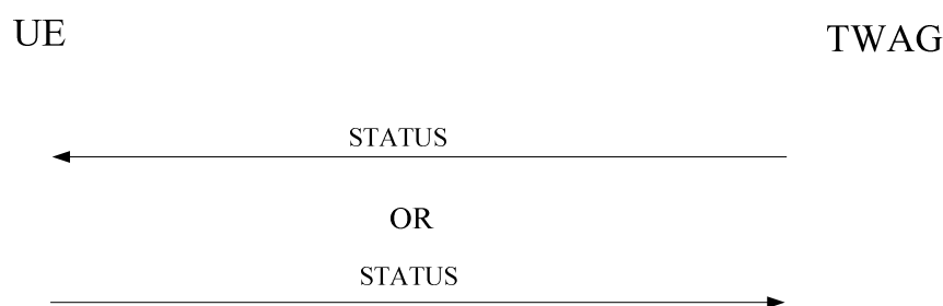
Figure 5.5.1: STATUS message
