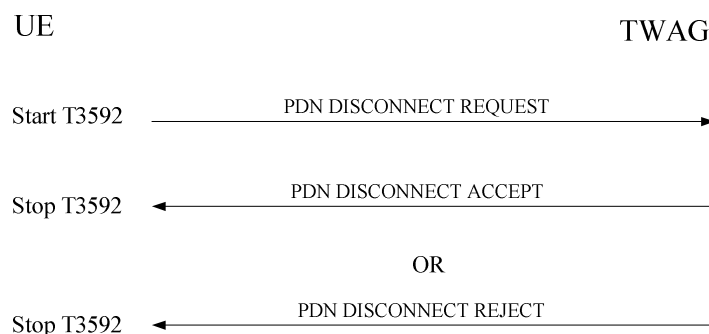
Figure 5.4.2.1: UE initiated PDN disconnection procedure
