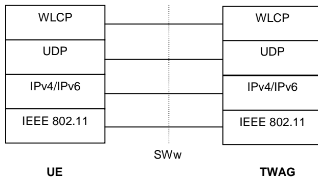
Figure 4.2.1: Protocol stack of WLCP
