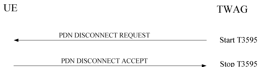
Figure 5.3.2.1: PDN disconnect procedure
