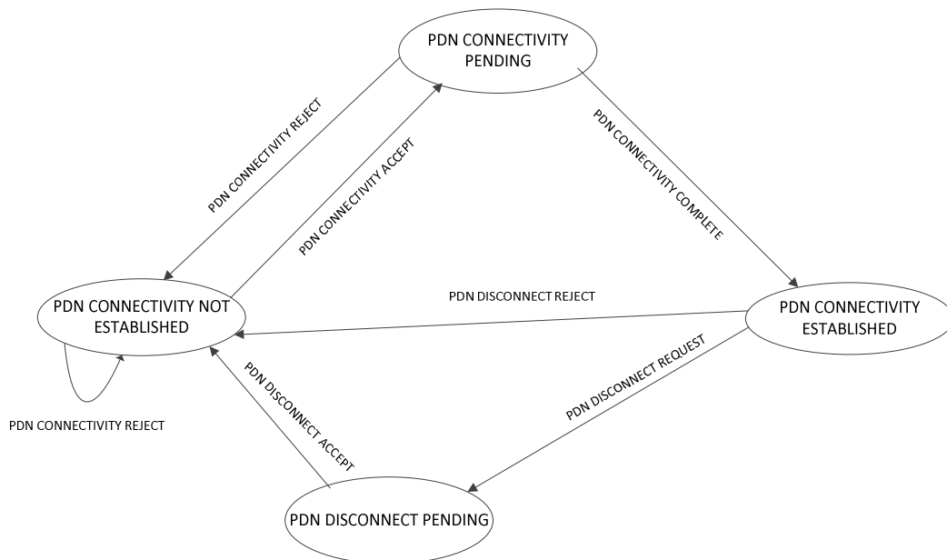
Figure 4.3.3.4.1: The WLCP states for PDN connectivity handling in the TWAG (overview)
