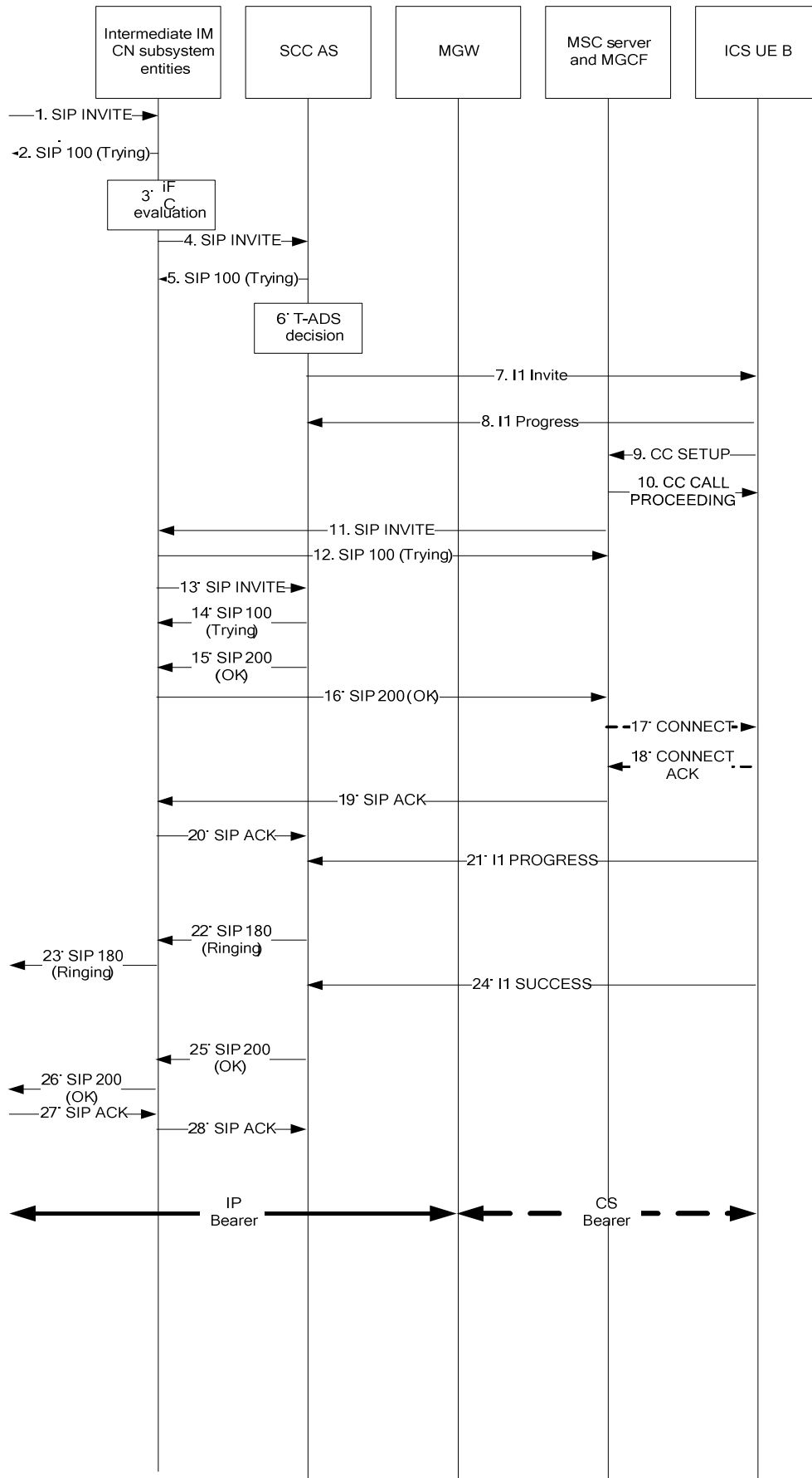
Figure A.5.7-1: ICS UE termination with CS media using Gm reference point when using an MSC server – network assisted T-ADS
