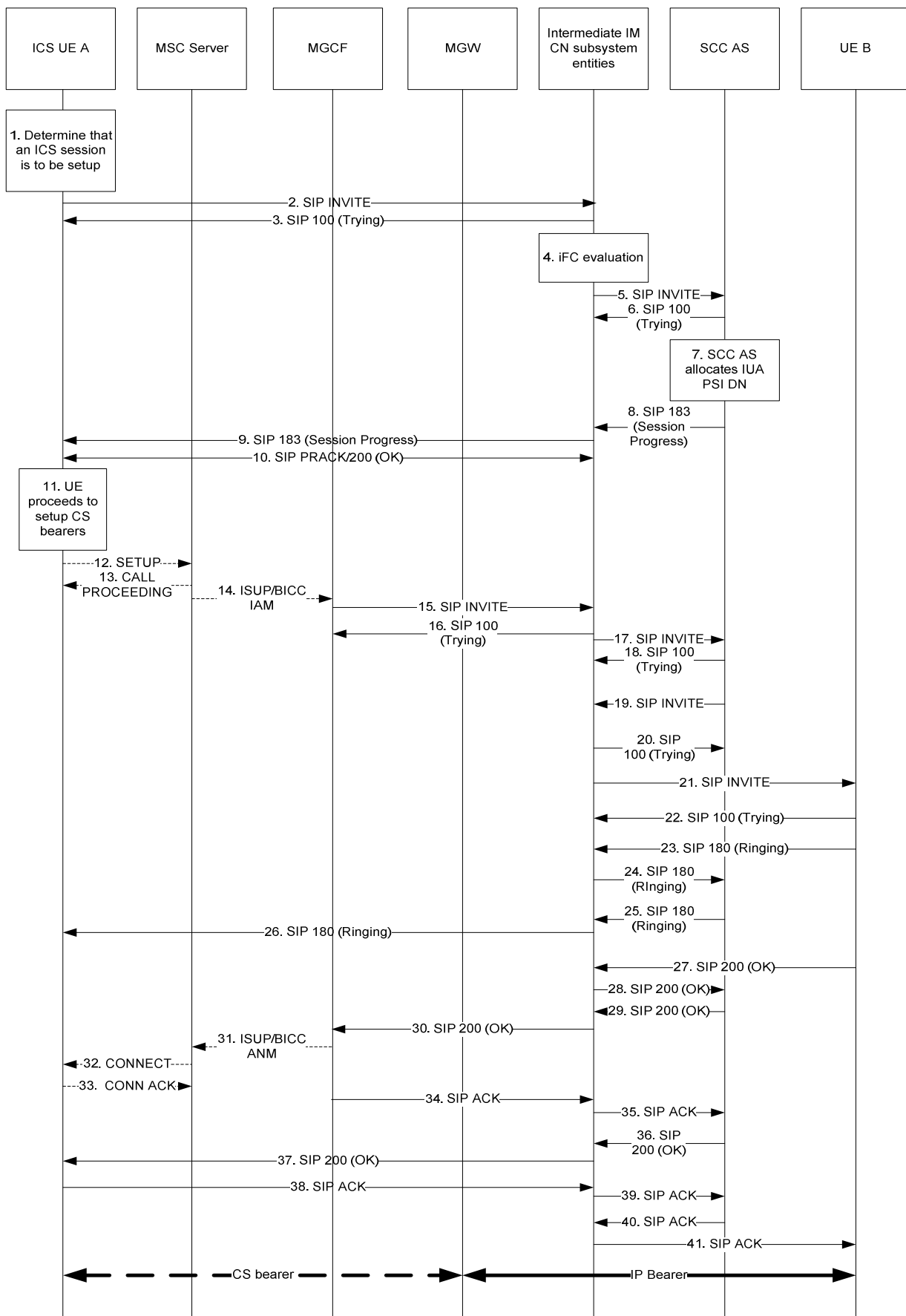
Figure A.4.2-1: ICS UE Origination with CS media using Gm reference point when using an MSC Server not enhanced for ICS
