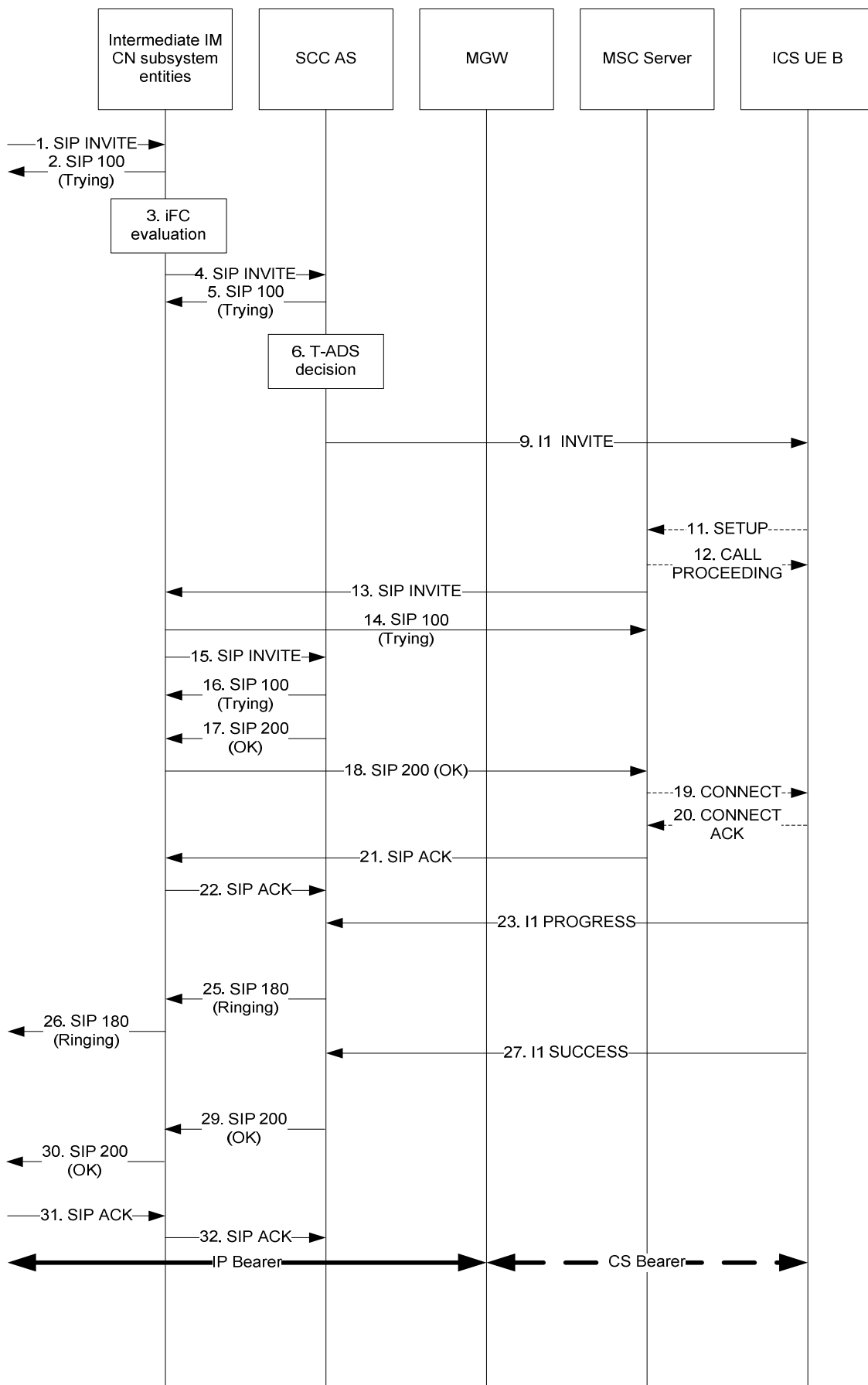
Figure A.5.6-1: ICS UE termination with CS media using Gm reference point when using an MSC Server enhanced for ICS
