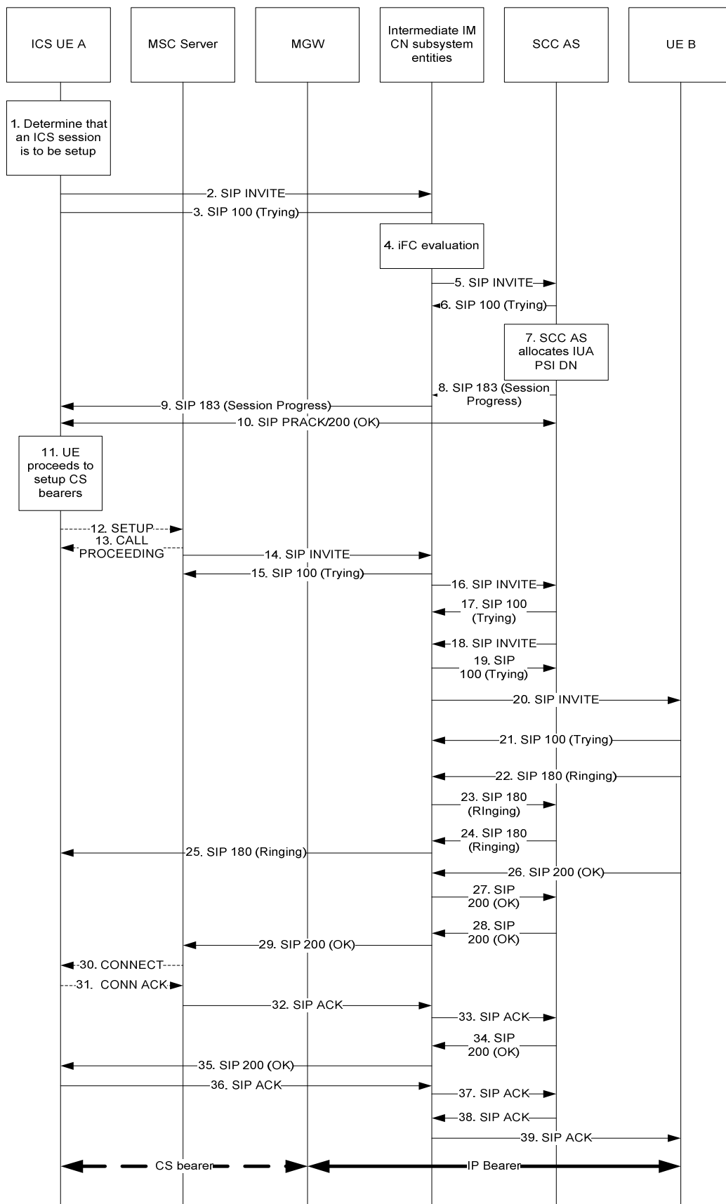
Figure A.4.1-1: ICS UE Origination with CS media using Gm reference point when using an MSC Server enhanced for ICS
