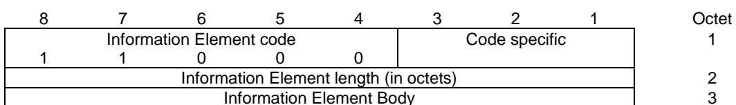
Figure 7.4.2.12.1: Mid-Call information element
