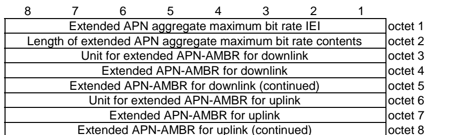
Figure 9.9.4.29.1: Extended APN aggregate maximum bit rate information element
