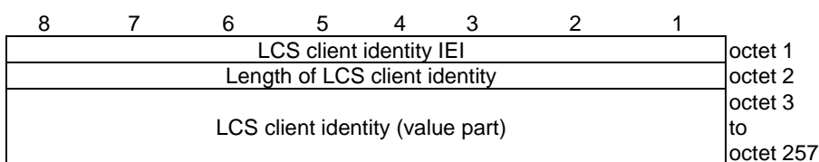
Figure 9.9.3.41.1: LCS client identity information element
