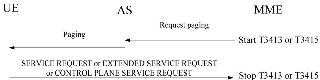
Figure 5.6.2.1.1: Paging procedure using S-TMSI
