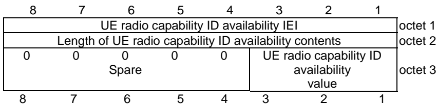
Figure 9.9.3.58.1: UE radio capability ID availability information element
