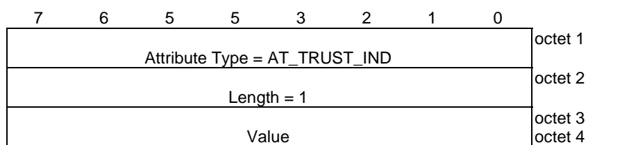
Figure 8.2.3.1-1: AT_TRUST_IND attribute
