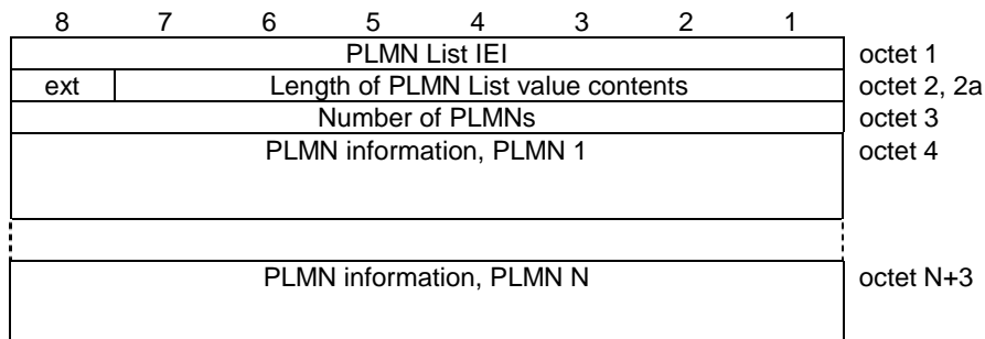
Figure H.2.4.2-1: PLMN List information element
